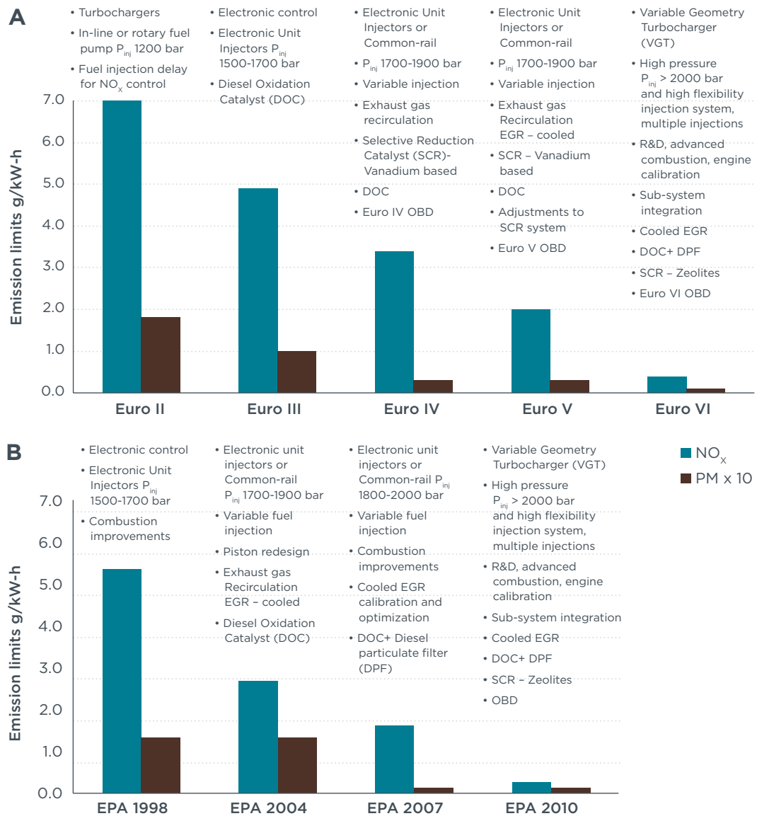
Figure 1. Progression of emission standard levels and adoption of new technologies for heavy-duty vehicles: a) European program; b) U.S. EPA program
