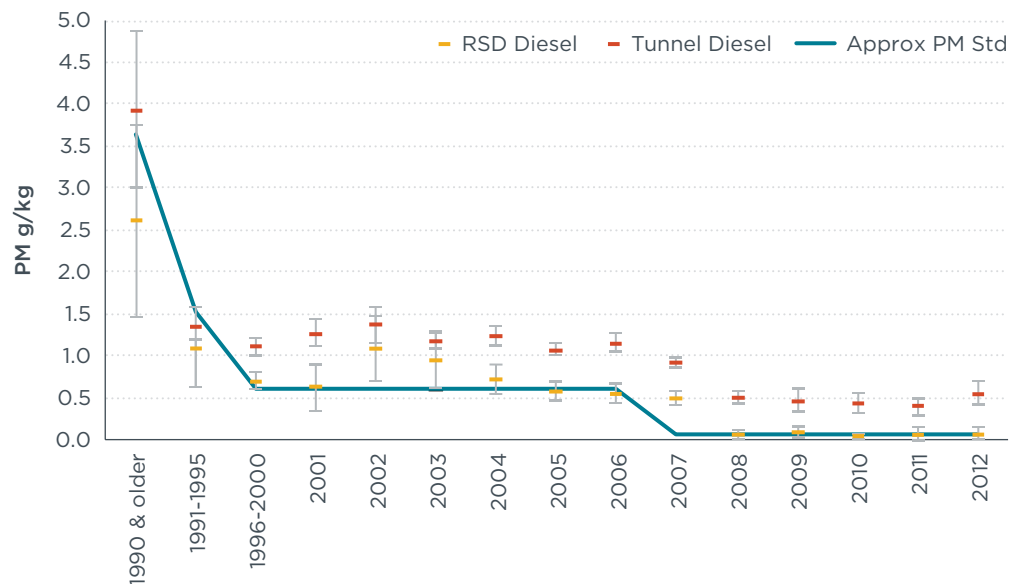
Figure 5. OHMS testing results for PM measurements of HDVs. OHMS (Tunnel) and RSD. Source: Envirotest Canada, 2013
