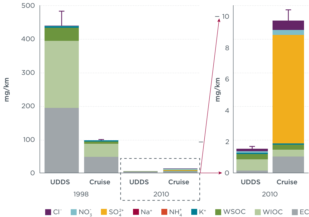
Figure 2. PM composition from a 1998 (uncontrolled, no after-treatment) and a 2010 heavy-duty truck. Note that the scale in the right panel (2010) has been magnified from the central panel to show the 2010 PM composition better. WSOC means water-soluble OC and WIOC means water-insoluble OC. UDDS stands for urban dynamometer driving schedule. Source: Ruehl et al., 2014.
