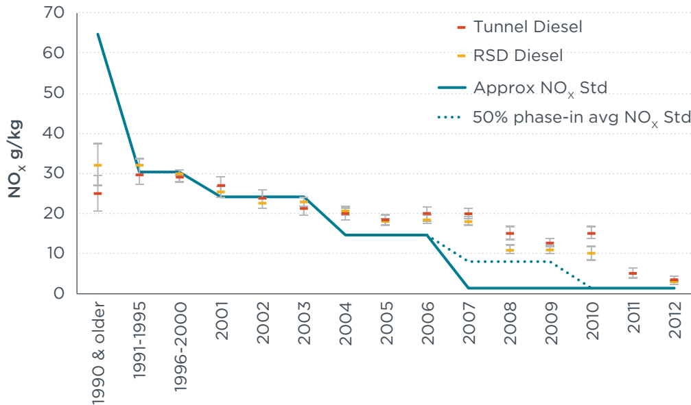
Figure 6. OHMS (Tunnel) and remote sensing device (RSD) NO x measurement for HDVs. Source: Envirotec Canada, 2013
