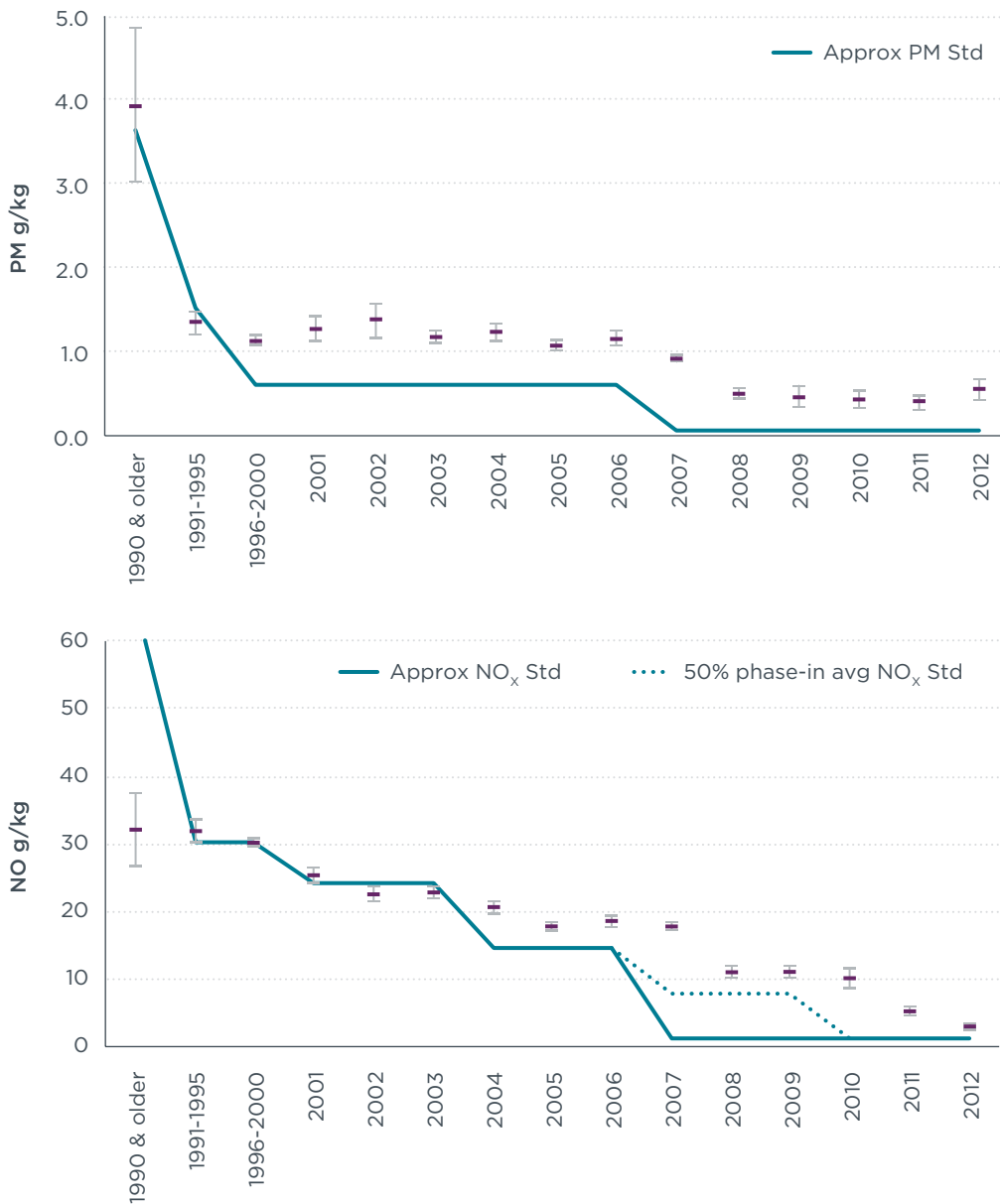
Figure 3. HDV PM and NO x emissions measurements with remote sensing devices (purple and blue markers). Source: Envirotec Canada, 2013
