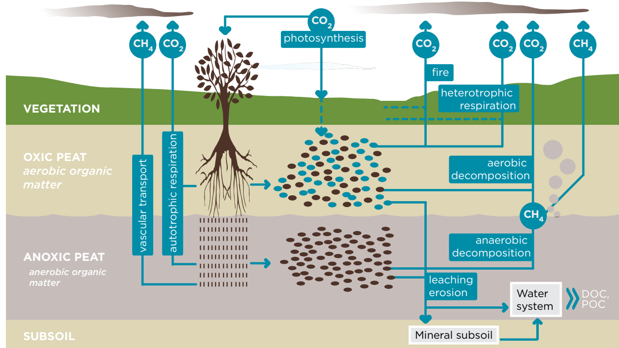
Figure 5: Schematic representation of carbon cycle processes, flow paths and stores in tropical peat (after Jauhiainen, Heikkinen, Martikainen, & Vasander, 2001).
