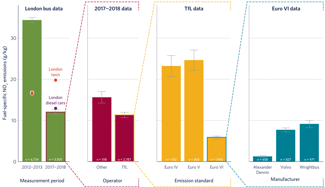
Average fuel-specific \text{NO}_x emissions from London buses. From left, results are shown by measurement period, operator, emission standard, and manufacturer.
