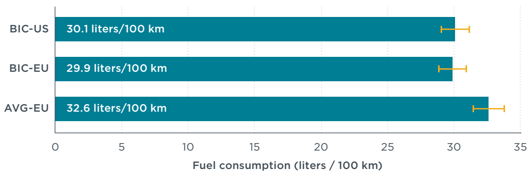
Figure 4. Measured fuel consumption on the chassis dynamometer over the EU Long Haul cycle. Error bars represent a 3% uncertainty associated with chassis dynamometer testing.
