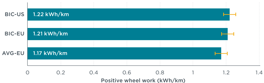
Figure 9. Distance-specific work applied by the chassis dynamometer on the wheels. Error bars are set to approximately 3%, representing only the impact of the uncertainties in aerodynamic testing. The uncertainty in the vehicle mass measurement is negligible. The same rolling resistance coefficient was used for all trucks.
