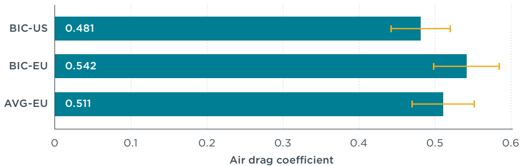
Figure 7. Air drag coefficient as measured by regulatory EU constant-speed test. Error bars are set to 7.5%, which is the tolerance allowed by the EU for the conformity of production testing of the air drag.
