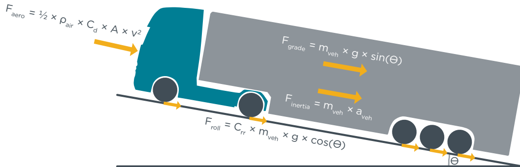
Figure 1. Road-load forces acting on a tractor-trailer.
