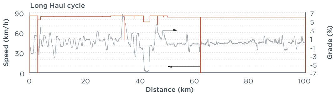
Figure 3. Vehicle speed target and road grade as a function of distance for the EU Long Haul cycle.
