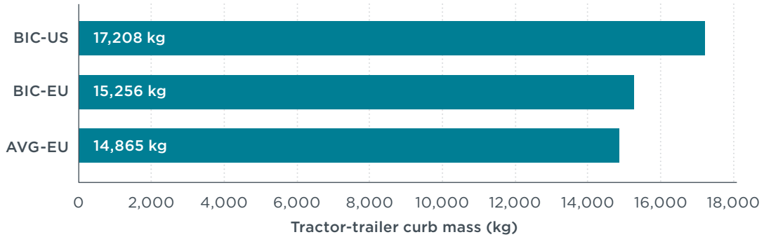
Figure 8. Curb mass of the tested tractors with 500 liters of fuel.
