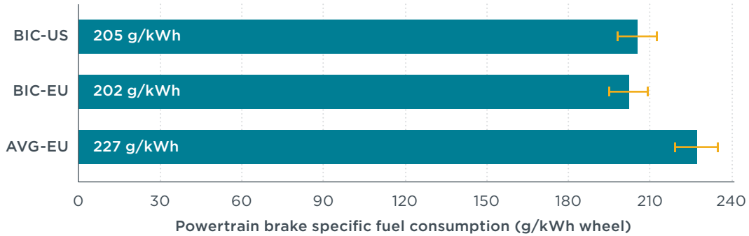
Figure 5. Powertrain efficiency, quantified as the measured fuel consumption per unit of work at the wheel. Error bars represent a 3% uncertainty associated with chassis dynamometer testing.
