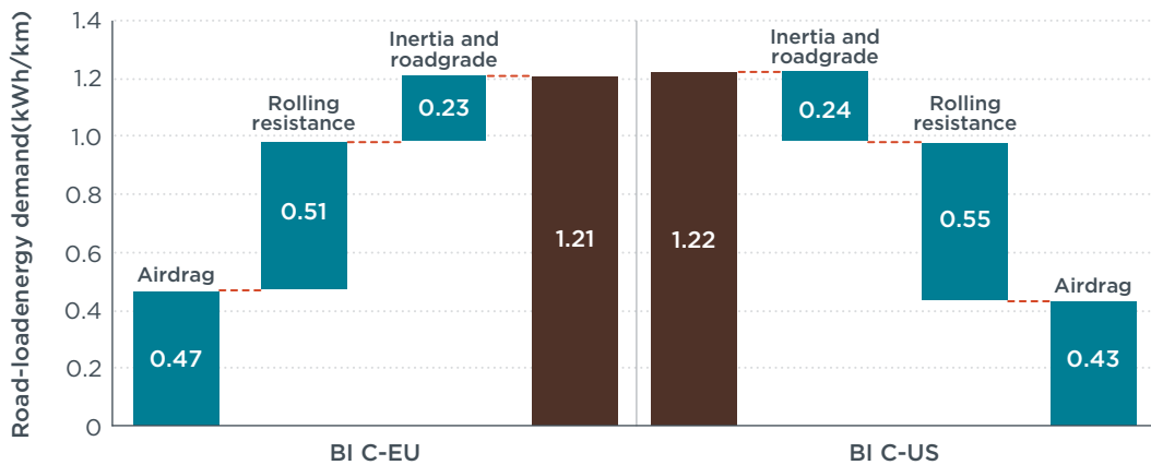
Figure 10. Individual contributions of components to the total road-load energy demand for the BIC-EU and BIC-US tractor-trailers over the EU Long Haul cycle.
