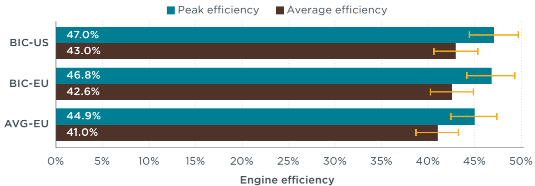
Figure 6. Average and peak efficiency estimated from the fuel consumption, as measured by the chassis dynamometer, and the work at the engine's crankshaft, as estimated from the CAN bus. Error bars represent a 5% uncertainty associated with the maximum inaccuracy expected from the CAN bus signals.
