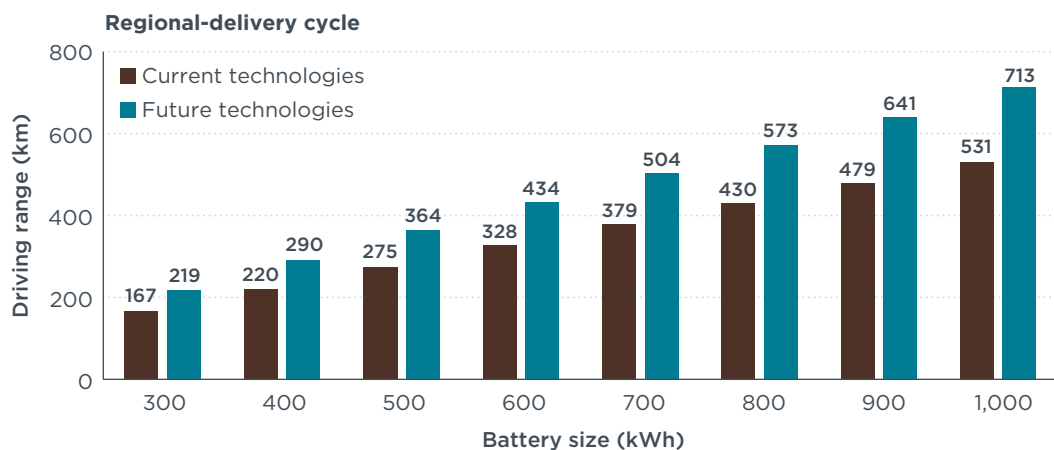
Figure 4. Driving range estimation for current and future technologies over the regional-delivery drive cycle using the reference payload.
