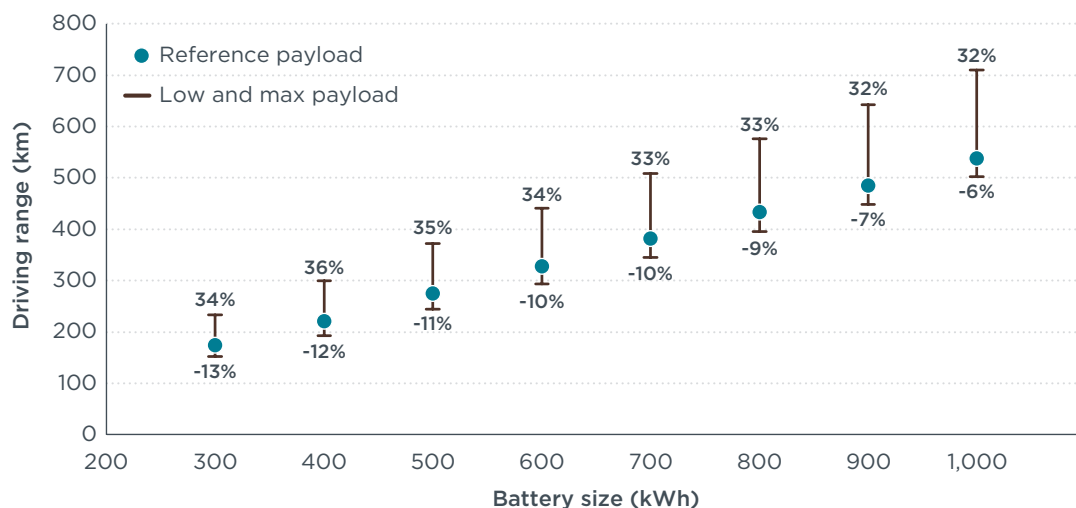
Figure 7. Impact of payload on tractor-trailer driving range over the long-haul cycle (reference payload: 19,300 kg).
