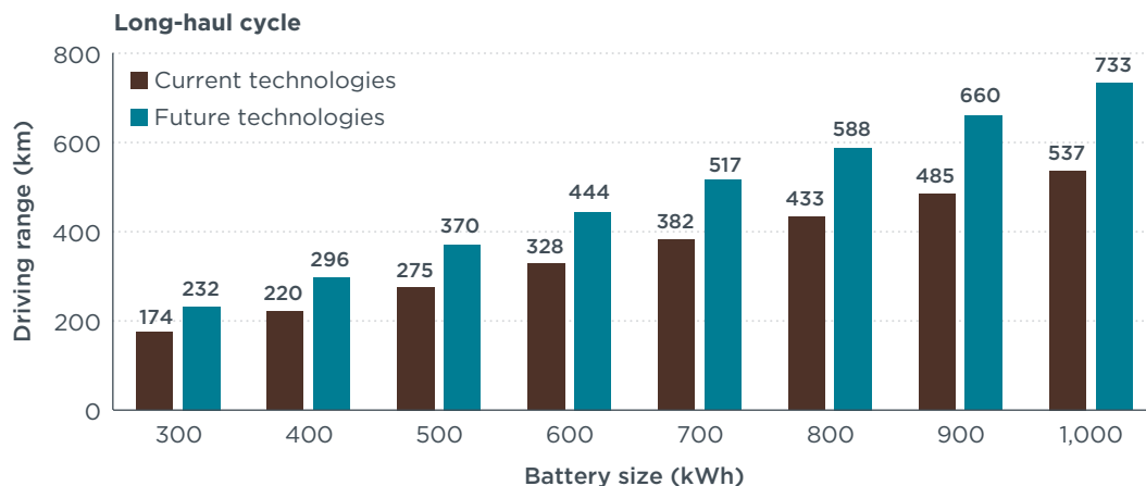
Figure 3. Driving range estimation for current and future technologies over the long-haul drive cycle using the reference payload.
