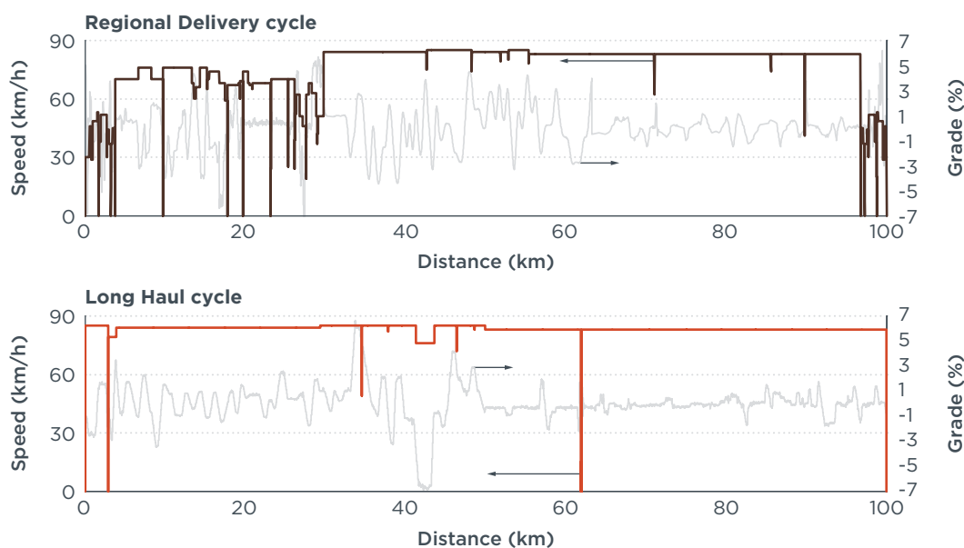
Figure 1. Long Haul and Regional Delivery VECTO cycles
