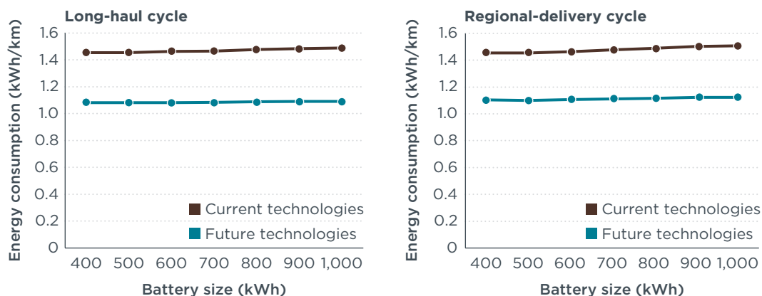
Figure 5. Energy consumption estimation for current and future technologies.
