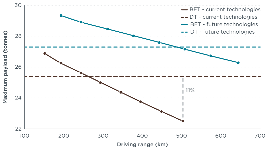
Figure 6. Maximum tractor-trailer payload as function of driving range.
