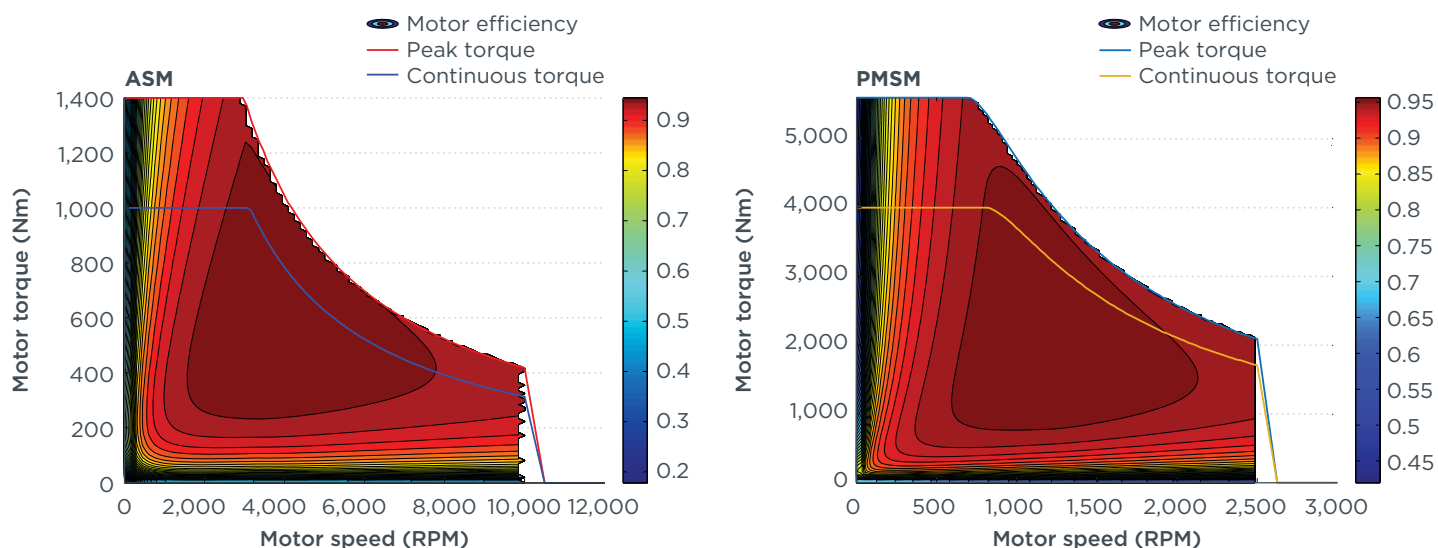
Figure 2. Efficiency map for the two types of electric motors at 800V operating voltage. ASM on the left and PMSM on the right.
