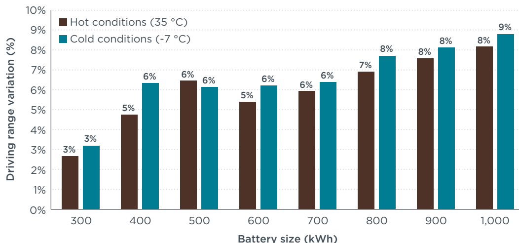
Figure 8: Driving range reduction at different ambient temperatures and battery sizes.
