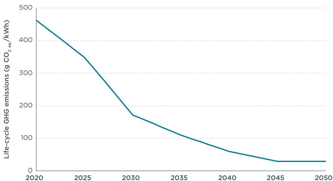
Figure 2.2. Development of the life-cycle GHG emission intensity of electricity consumption in Germany in the carbon neutral 2045 scenario.
