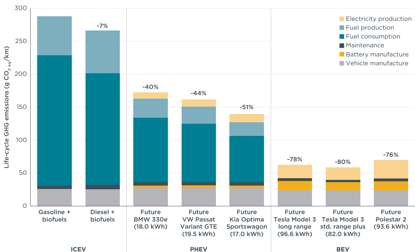
Figure 3.9. Life-cycle GHG emissions of hypothetical future versions of the selected medium segment PHEV and BEV models compared to average medium segment gasoline and diesel ICEVs driven in Germany in 2030 to 2047.
