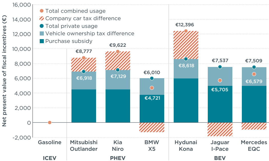
Figure 3.13. Net present value of the fiscal incentives for selected SUV segment PHEV and BEV models for a purchase in 2021. The difference in the vehicle ownership tax (over 18 years) and company car taxation (over 2 years) corresponds to a segment average gasoline ICEV.
