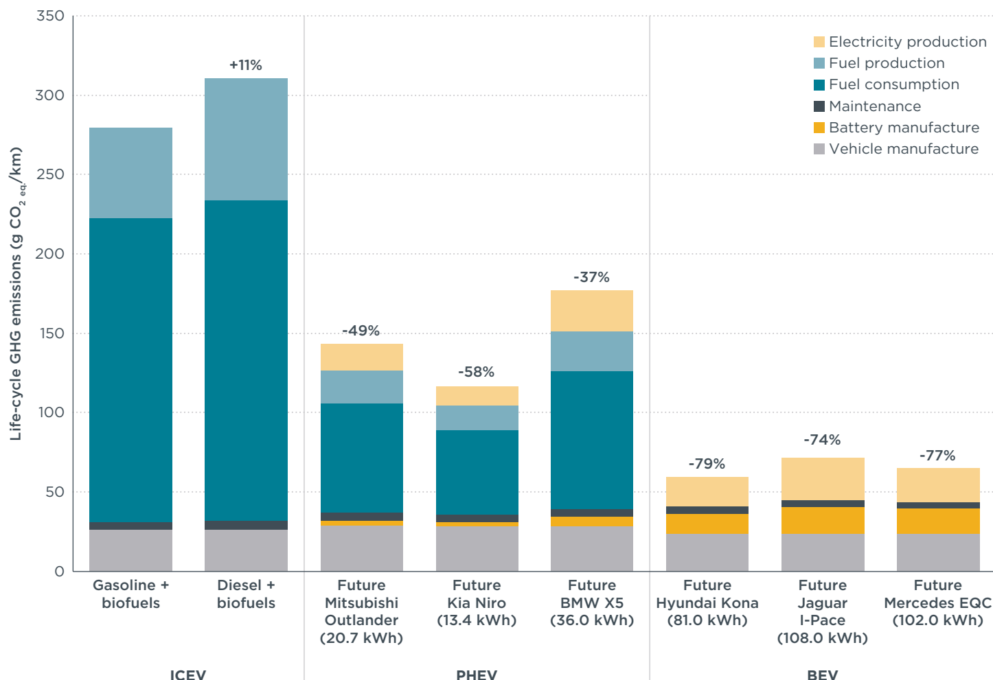
Figure 3.10. Life-cycle GHG emissions of hypothetical future versions of the selected SUV segment PHEV and BEV models compared to average SUV segment gasoline and diesel ICEVs driven in Germany in 2030 to 2047.
