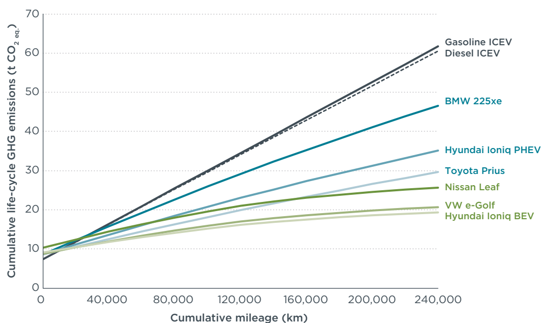
Figure 3.5. Cumulative life-cycle GHG emissions over the lifetime of selected PHEV and BEV models compared to average lower medium segment gasoline and diesel ICEVs driven in Germany in 2021 to 2038.
