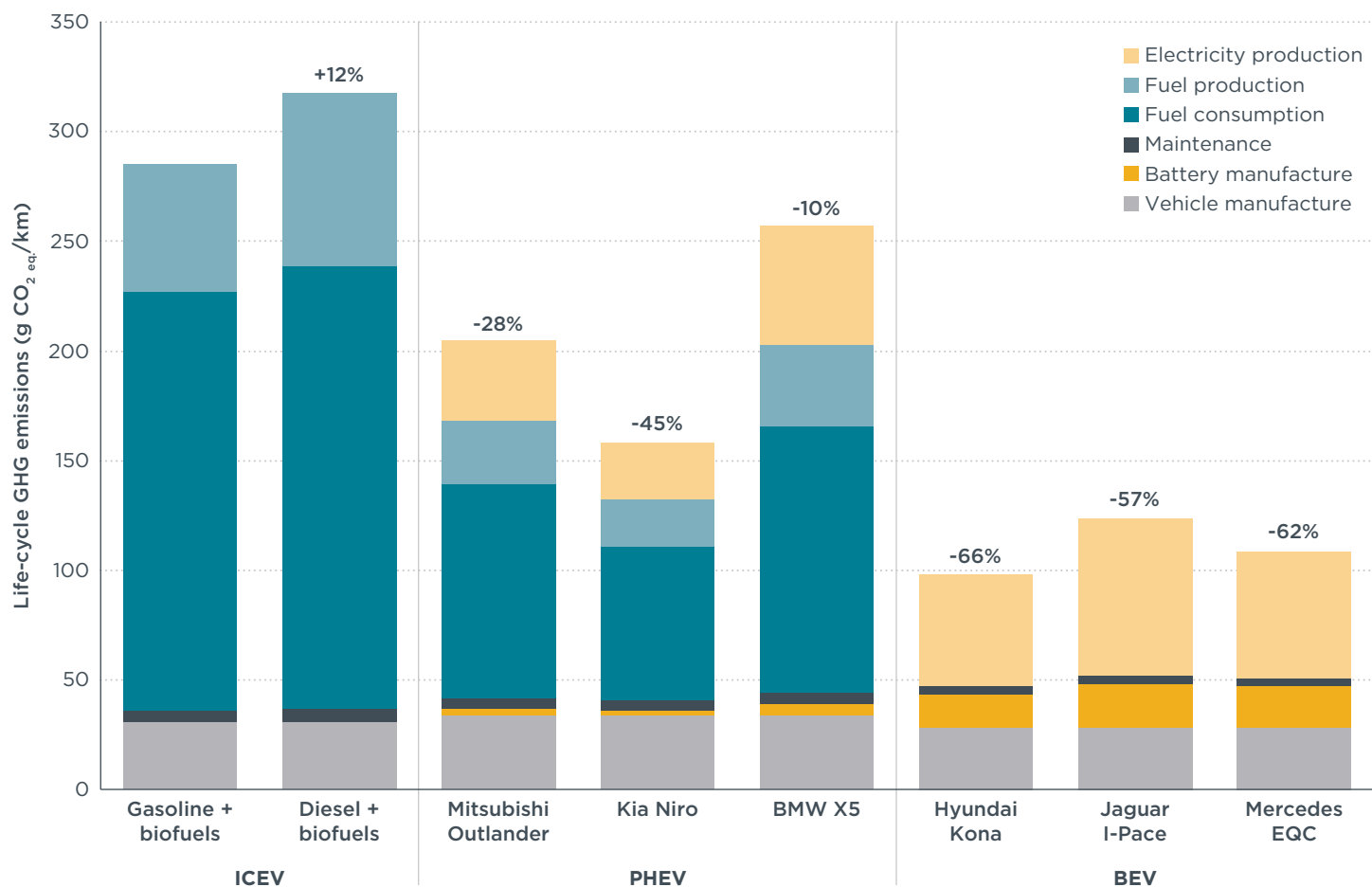
Figure 3.3. Life-cycle GHG emissions of selected SUV segment PHEV and BEV models compared to average SUV segment gasoline and diesel ICEVs driven in Germany in 2021 to 2038.
