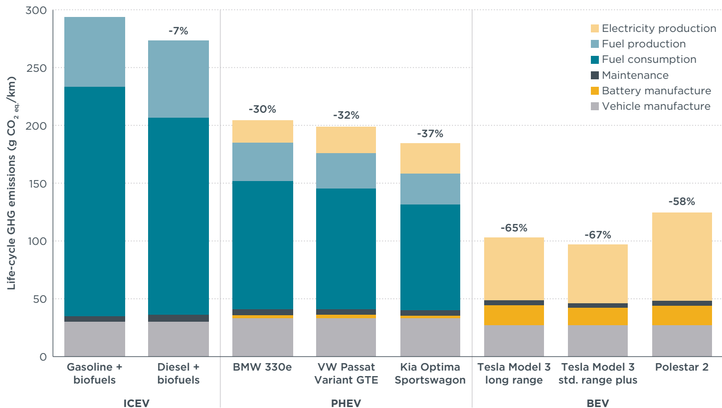
Figure 3.2. Life-cycle GHG emissions of selected medium segment PHEV and BEV models compared to average medium segment gasoline and diesel ICEVs driven in Germany in 2021 to 2038.
