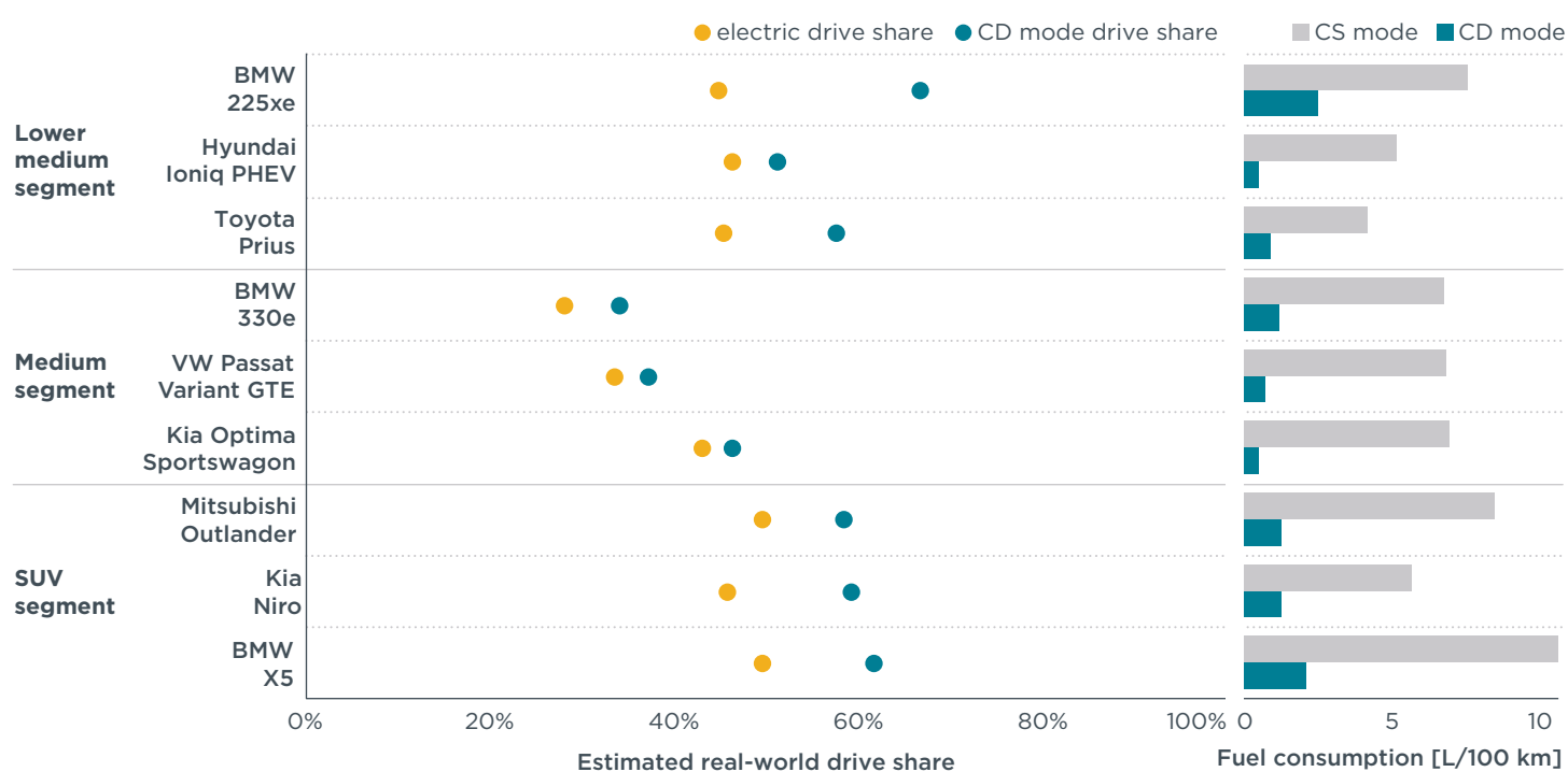
Figure 2.1. Estimated electric and CD mode drive shares of the selected PHEV models (left), and fuel consumption in CS and CD mode (right).
