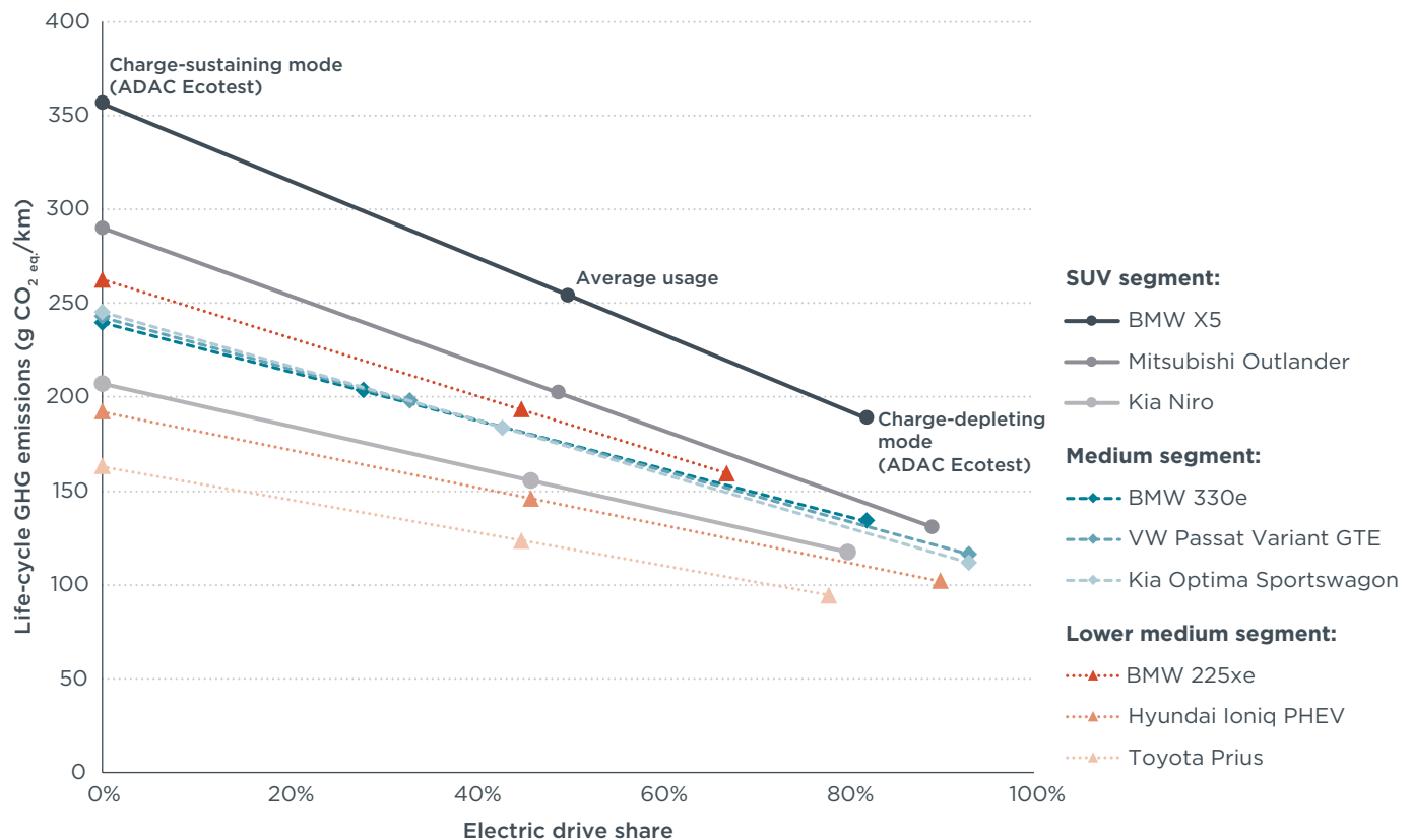
Figure 3.4. Life-cycle GHG emissions of selected SUV (solid), medium (dashed) and lower medium segment (dotted) PHEV models as a function of the electric drive share. The emissions corresponding to the average usage of private cars, solely driving in charge-sustaining mode, and solely driving in charge-depleting mode are highlighted.
