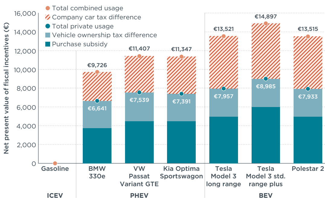
Figure 3.12. Net present value of the fiscal incentives for selected medium segment PHEV and BEV models for a purchase in 2021. The difference in the vehicle ownership tax (over 18 years) and company car taxation (over 2 years) corresponds to a segment average gasoline ICEV.
