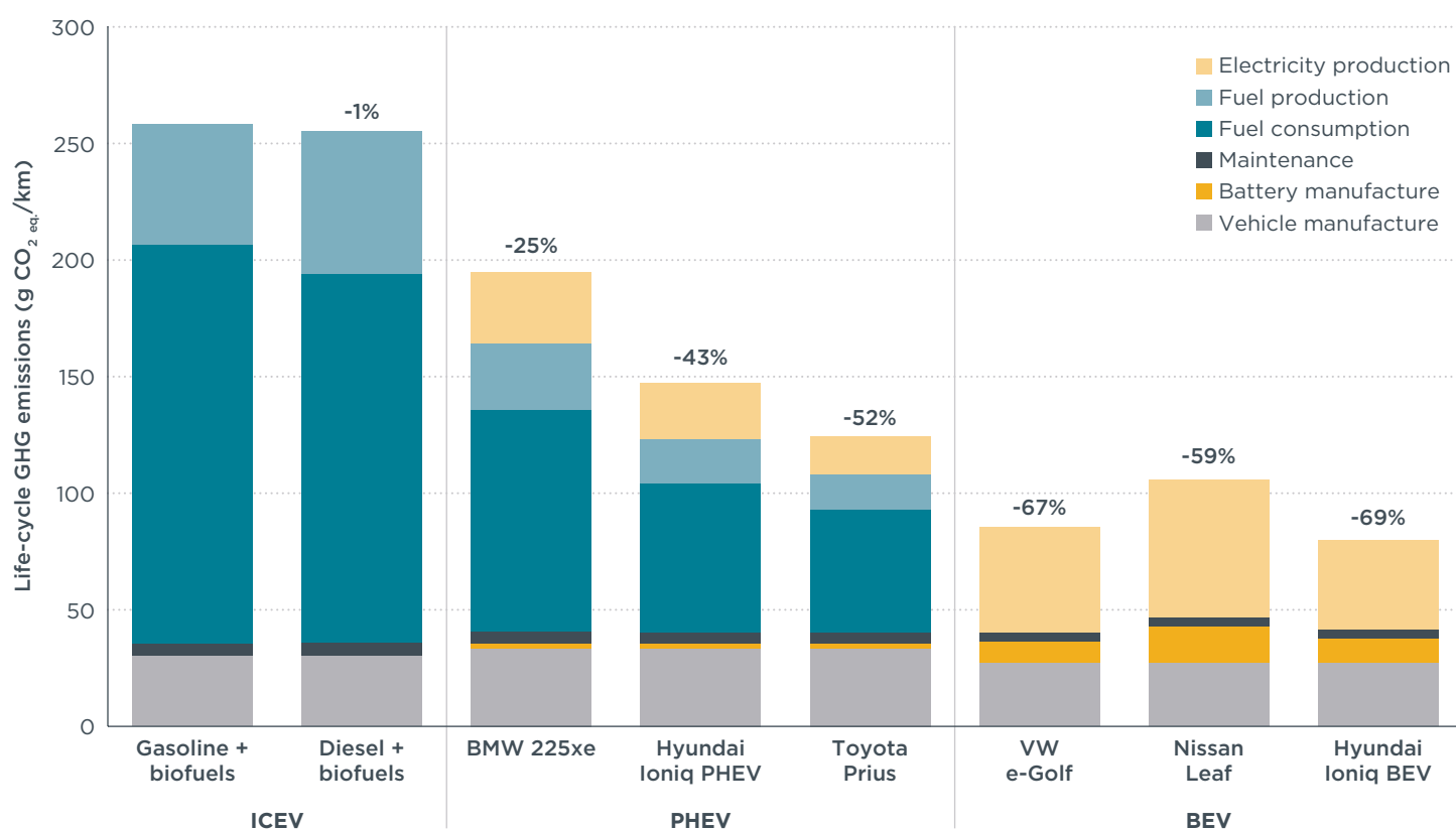
Figure 3.1. Life-cycle GHG emissions of selected lower medium segment PHEV and BEV models compared to average lower medium segment gasoline and diesel ICEVs driven in Germany in 2021 to 2038.
