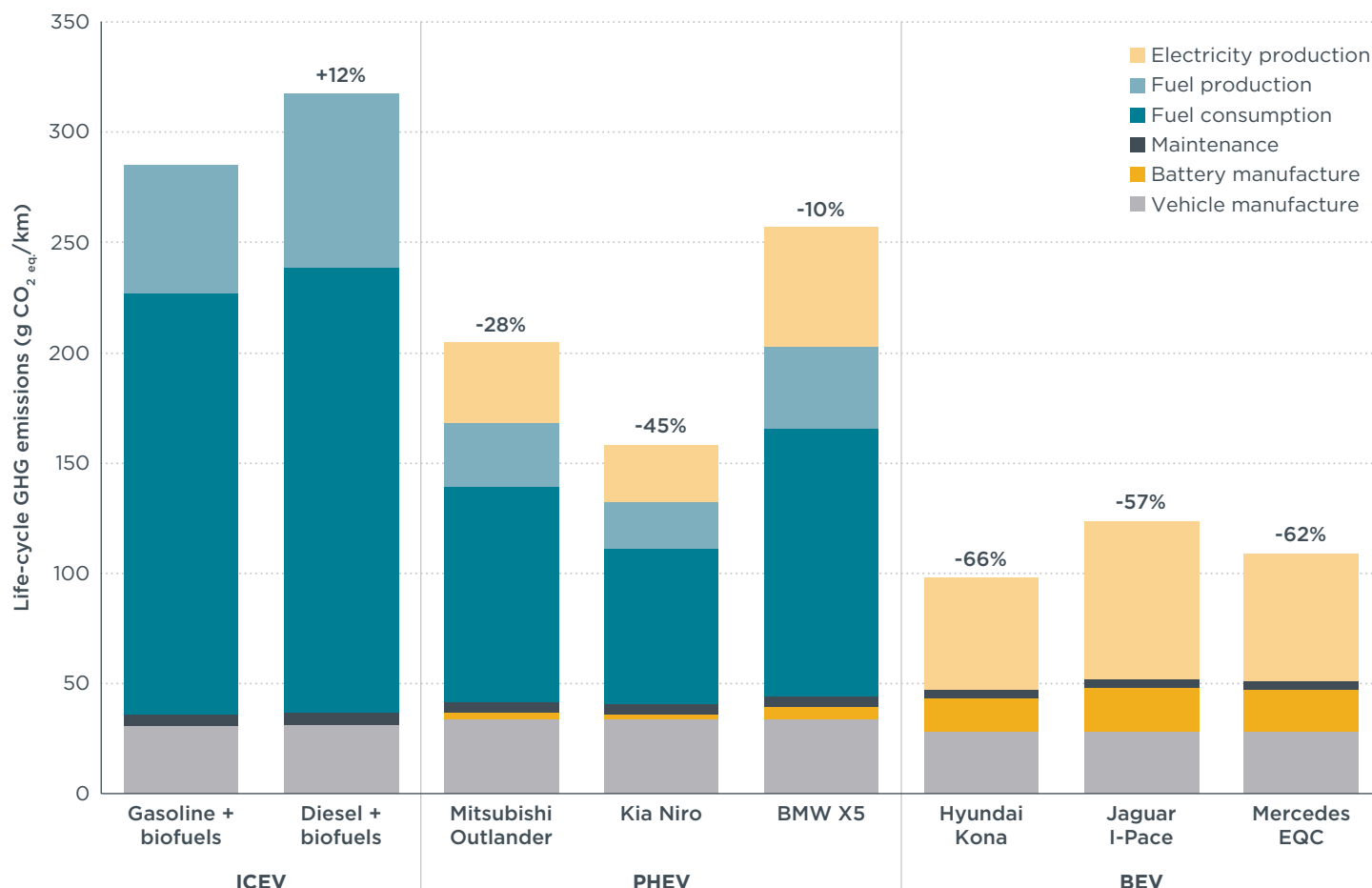
Figure ES1. Life-cycle GHG emissions of selected SUV segment PHEV and BEV models compared to average SUV segment gasoline and diesel ICEVs driven in Germany in 2021 to 2038.
