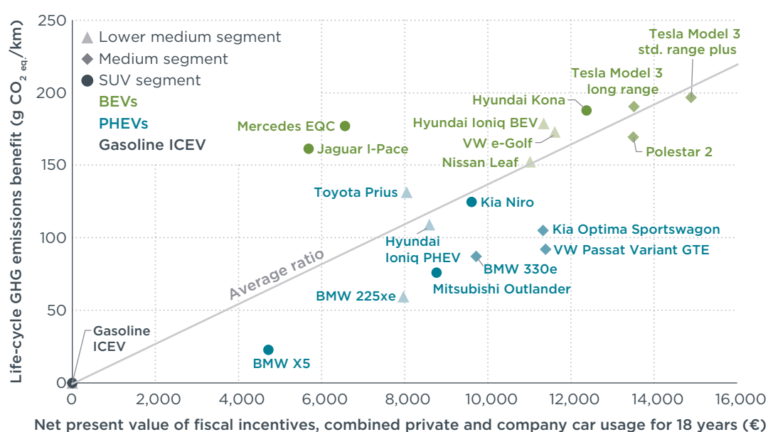
Figure 3.17. Life-cycle GHG emissions benefit when compared to a segment average gasoline ICEV versus net present value of the fiscal incentives for the PHEV and BEV models in combined company car and private usage in 2021 to 2038.
