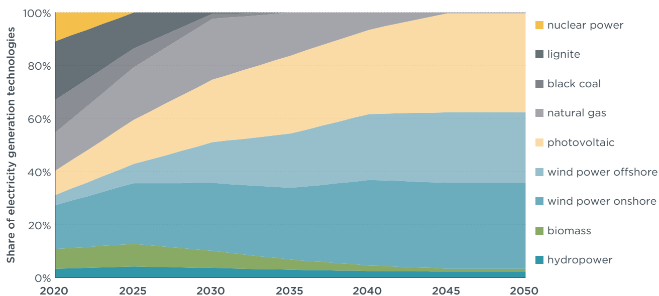
Figure A1. Projected shares of the electricity generation technologies in net electricity generation in Germany.
