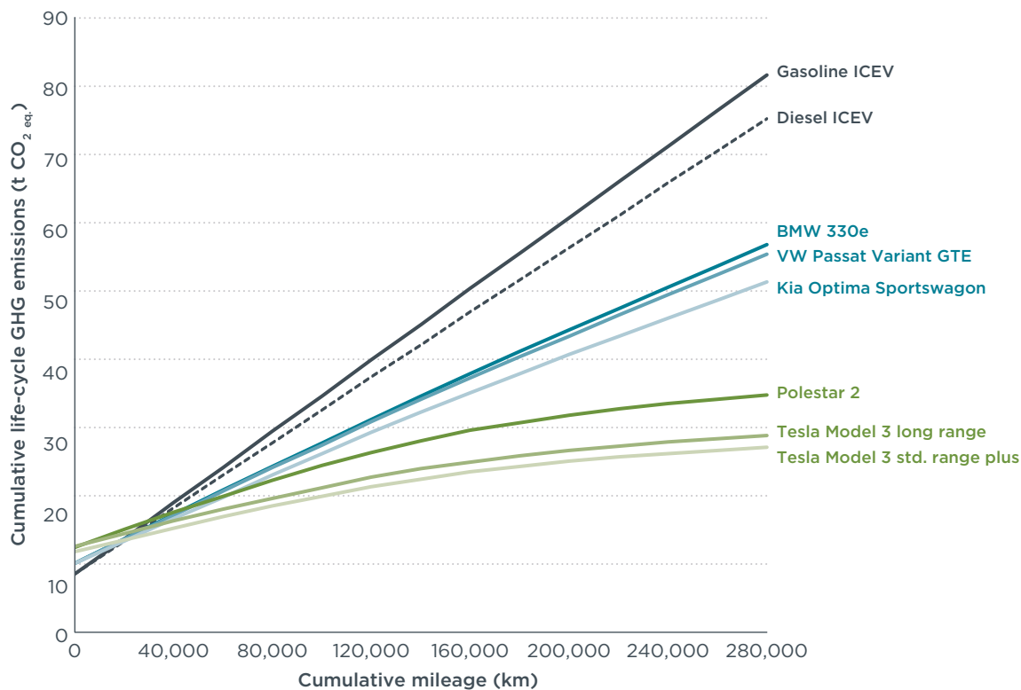
Figure 3.6. Cumulative life-cycle GHG emissions over the lifetime of selected PHEV and BEV models compared to average medium segment gasoline and diesel ICEVs driven in Germany in 2021 to 2038.
