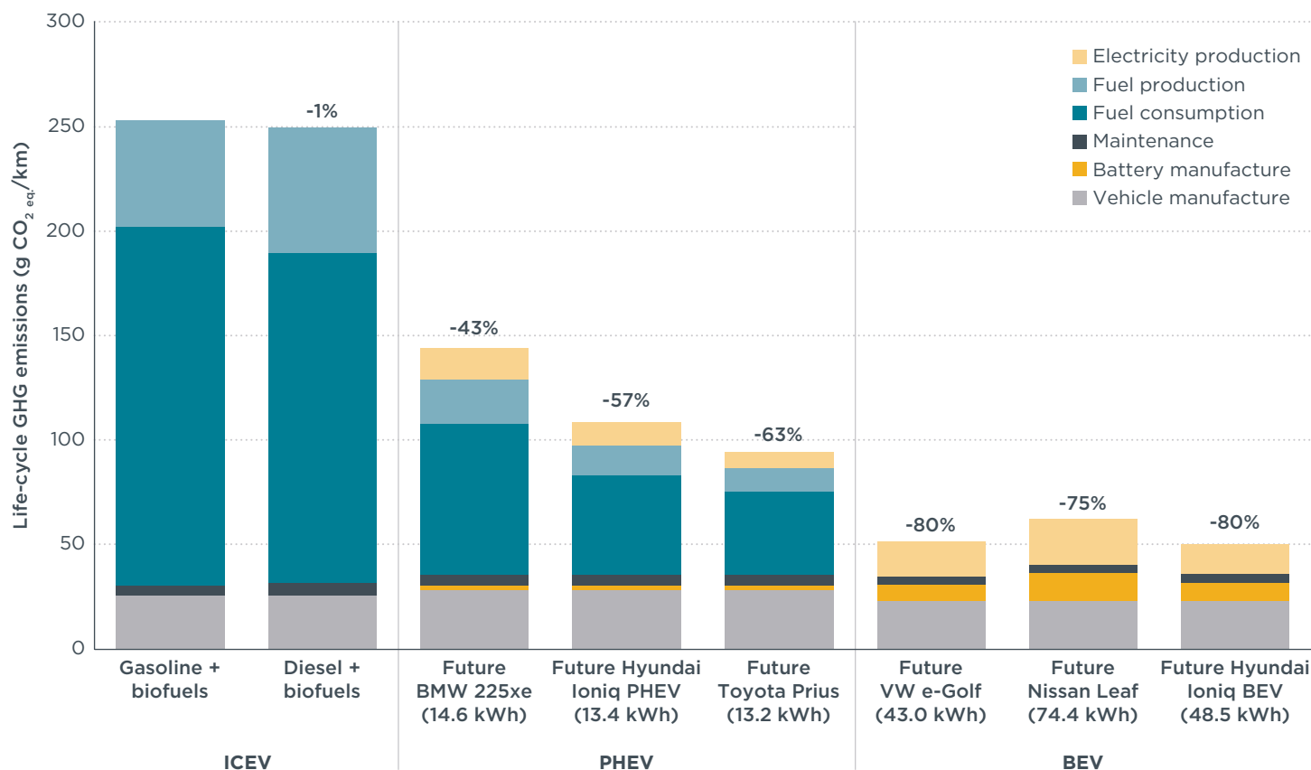
Figure 3.8. Life-cycle GHG emissions of hypothetical future versions of the selected lower medium segment PHEV and BEV models compared to average lower medium segment gasoline and diesel ICEVs driven in Germany in 2030 to 2047.
