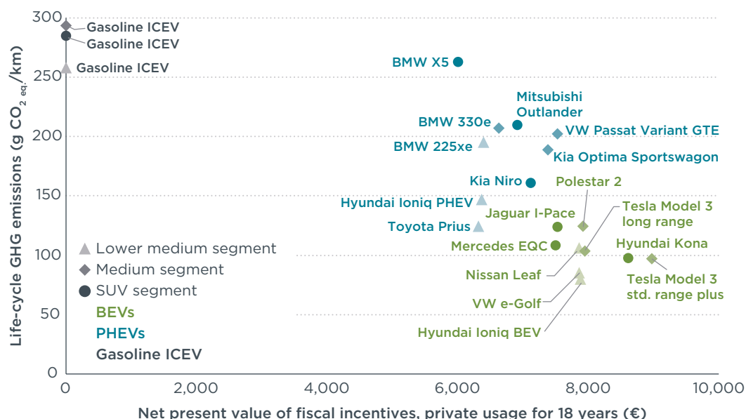
Figure 3.14. Life-cycle GHG emissions versus net present value of the fiscal incentives for the PHEV and BEV models in private usage in 2021 to 2038.
