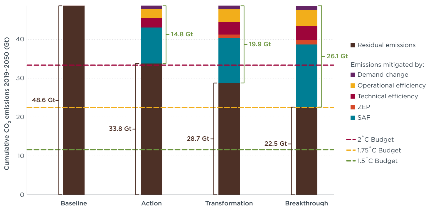
Figure ES-2. Cumulative global aviation CO 2 emissions by scenario and measure, 2019-2050
