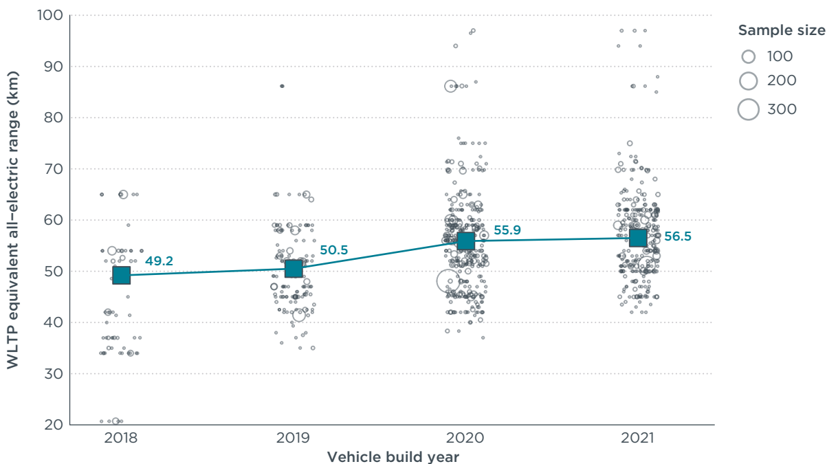
Figure 8. Development of the WLTP equivalent all-electric range (EAER) per vehicle build year of PHEVs in the WLTP sample.
