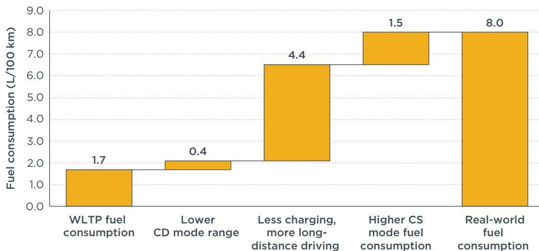
Figure 10. Contribution of different factors to real-world fuel consumption of company car PHEVs.
