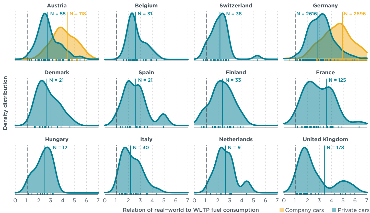
Figure ES2. Distribution of real-world fuel consumption values in relation to WLTP type-approval fuel consumption values for PHEVs across Europe. ‘N’ indicates the number of vehicles included in the respective sample. Solid vertical bars indicate country specific (sample size-weighted) mean, dashed vertical lines correspond to where the real-world and type-approval values are the same.
