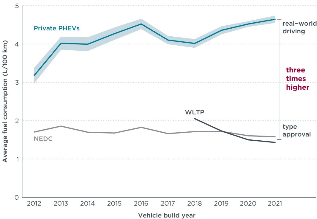
Figure 1. Development of the average real-world and type-approval fuel consumption of private PHEVs in Europe over vehicle build year. Shaded area indicates 95% confidence intervals for the mean.
