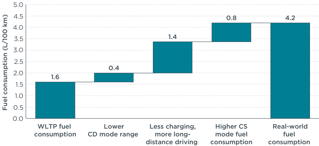
Figure 9. Contribution of different real-world factors to real-world fuel consumption of private car PHEVs.
