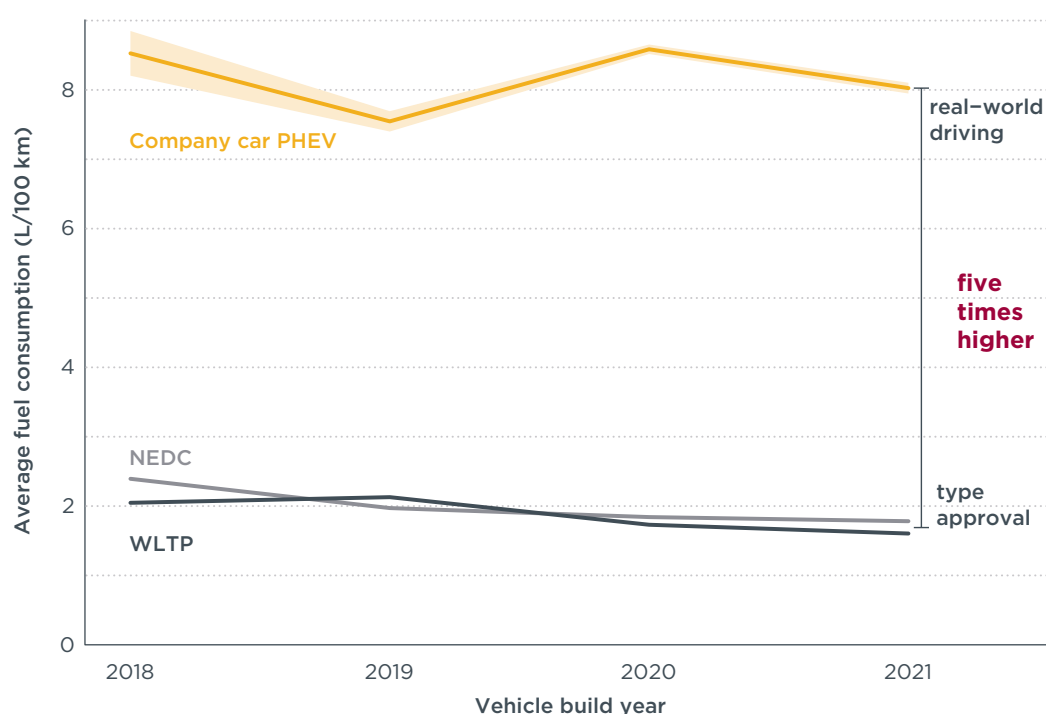
Figure 2. Development of the average real-world and type-approval fuel consumption of company car PHEVs in Europe over vehicle build year. Shaded area indicates 95% confidence intervals for the mean.
