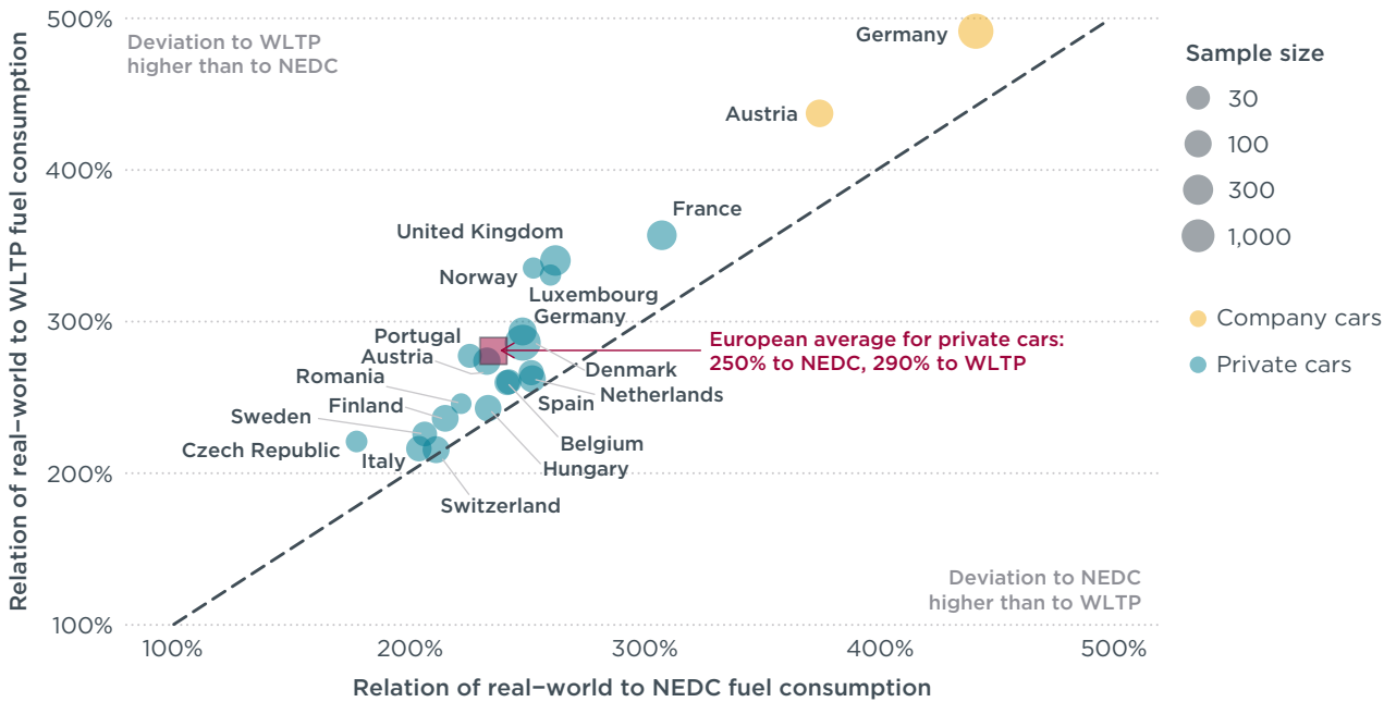
Figure 5. Mean relation of real-world to NEDC and WLTP type-approval fuel consumption by country sample.
