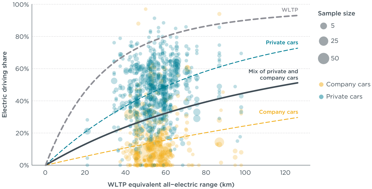
Figure 6. Real-world electric driving share of WLTP type-approved PHEVs compared to WLTP assumption on charge-depleting mode driving share and real-world adjusted UF curves.
