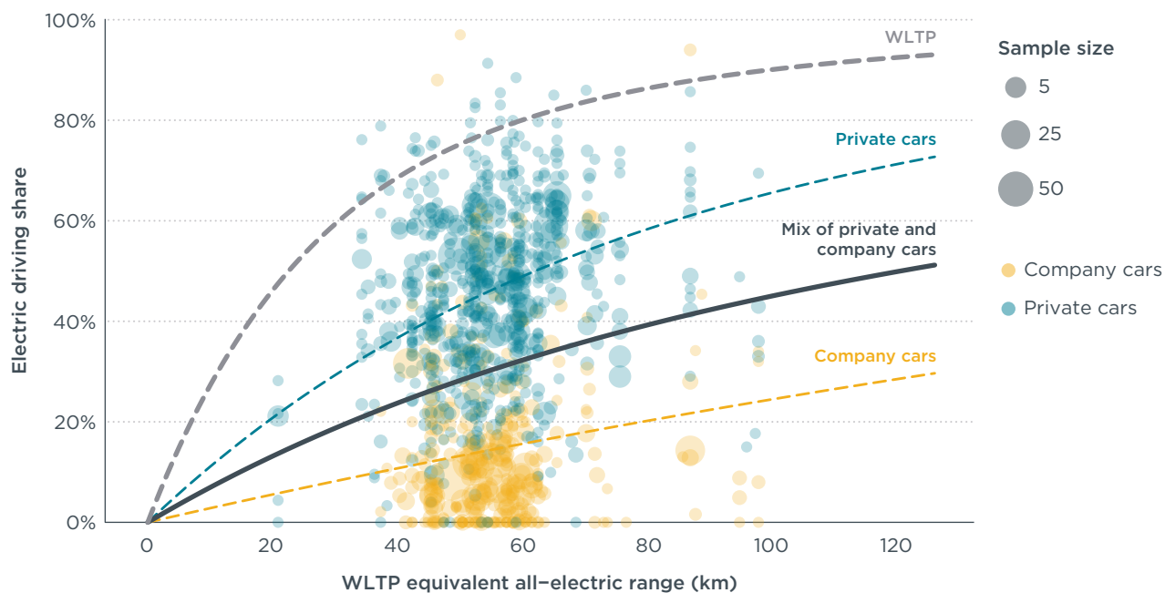
Figure ES3. Real-world electric driving share compared to WLTP assumption on charge-depleting mode driving share.
