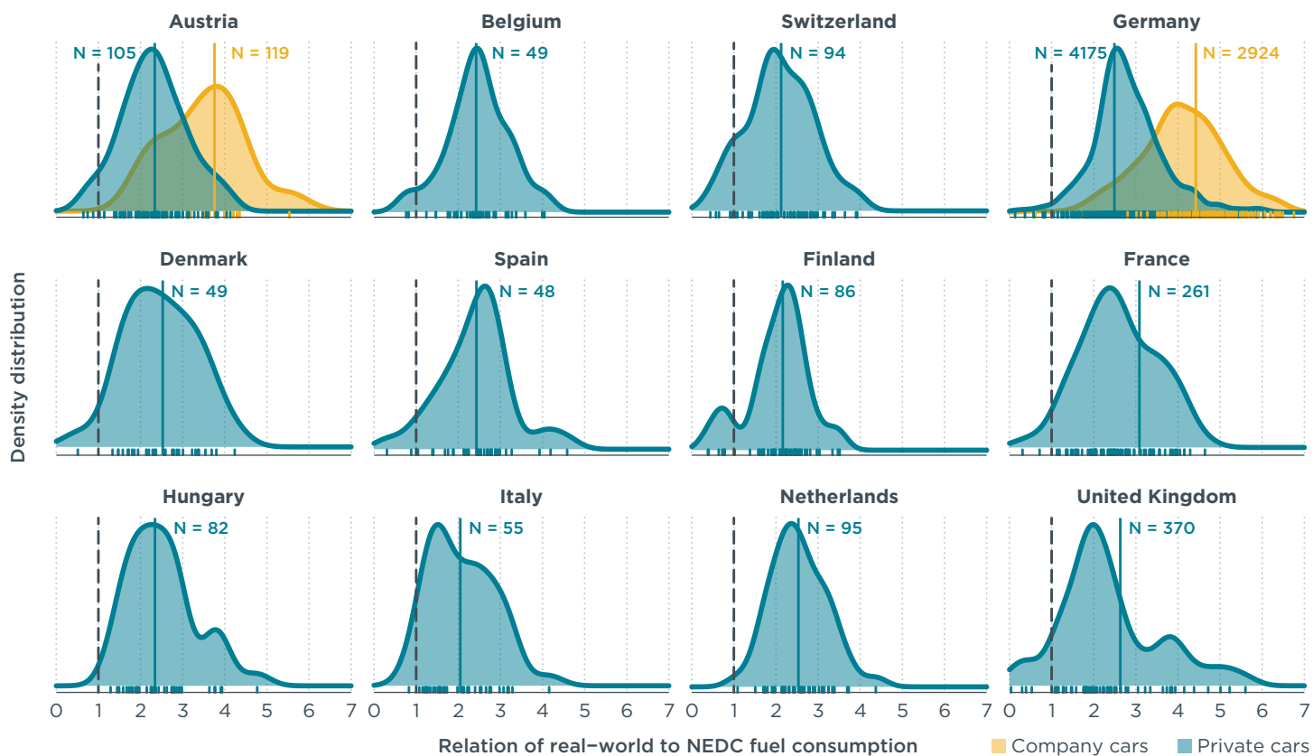
Figure 3. Distribution of real-world fuel consumption in relation to NEDC fuel consumption by country. The vertical dashed lines correspond to vehicles where the real-world and type-approval fuel consumption are the same. Thin colored vertical lines indicate the mean deviation by country and user group. Small rugs below the x-axis indicate individual observations at model variant level.
