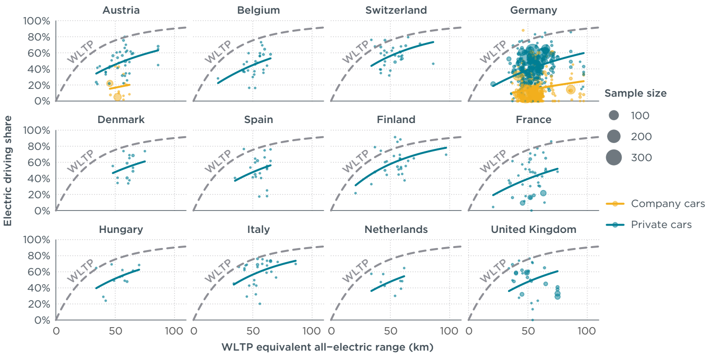
Figure 7. Real-world electric driving share of WLTP type-approved PHEVs compared to WLTP assumption on charge-depleting mode driving share and real-world adjusted UF curves for individual country samples.
