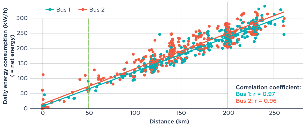
Figure 4. Relationship between energy consumption and daily distance
