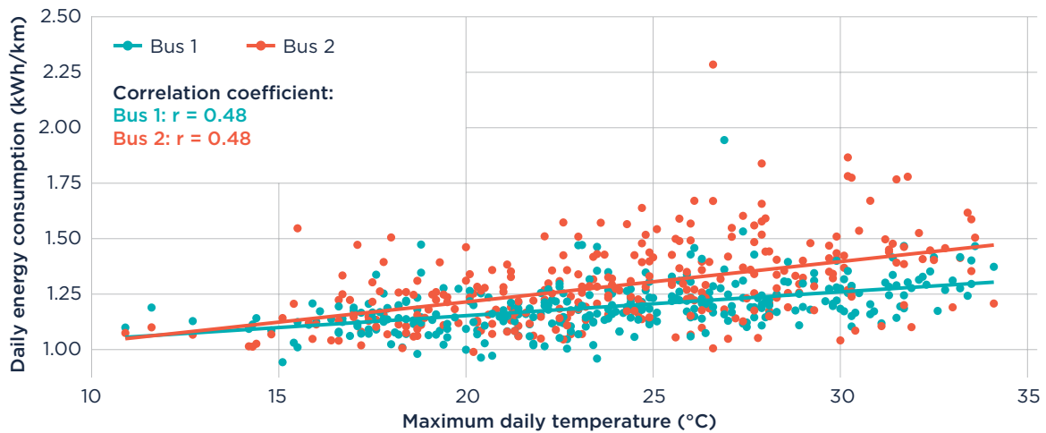
Figure 8. Relationship between daily energy consumption per kilometer by maximum daily temperature (in Celsius)
