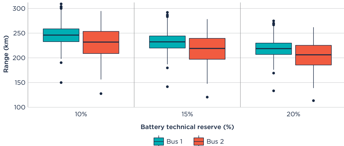
Figure 15. Range estimates for three battery technical reserve scenarios (10%, 15%, and 20%)
