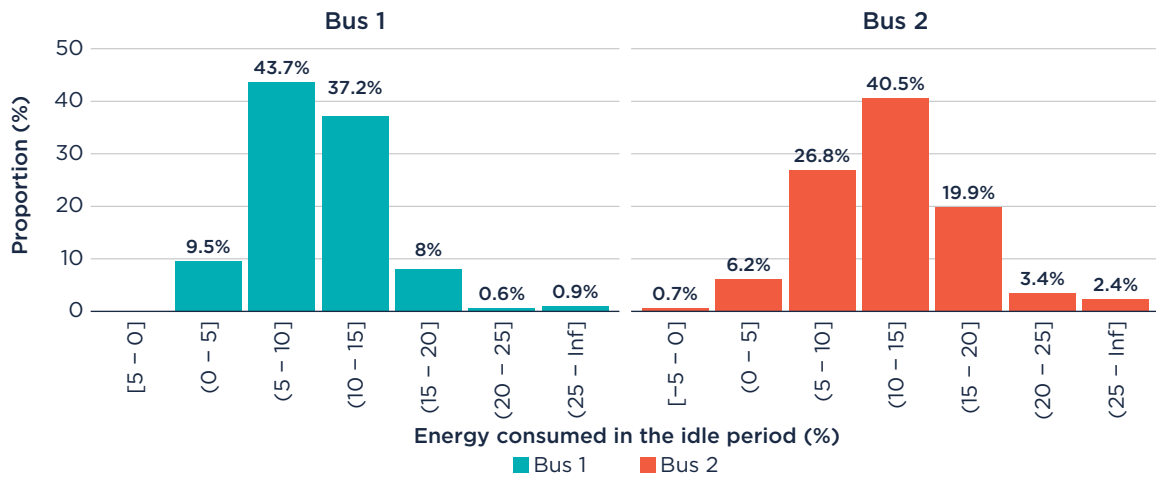
Figure 12. Distribution of the percentage of energy consumed per day in the idle period by the two monitored buses
