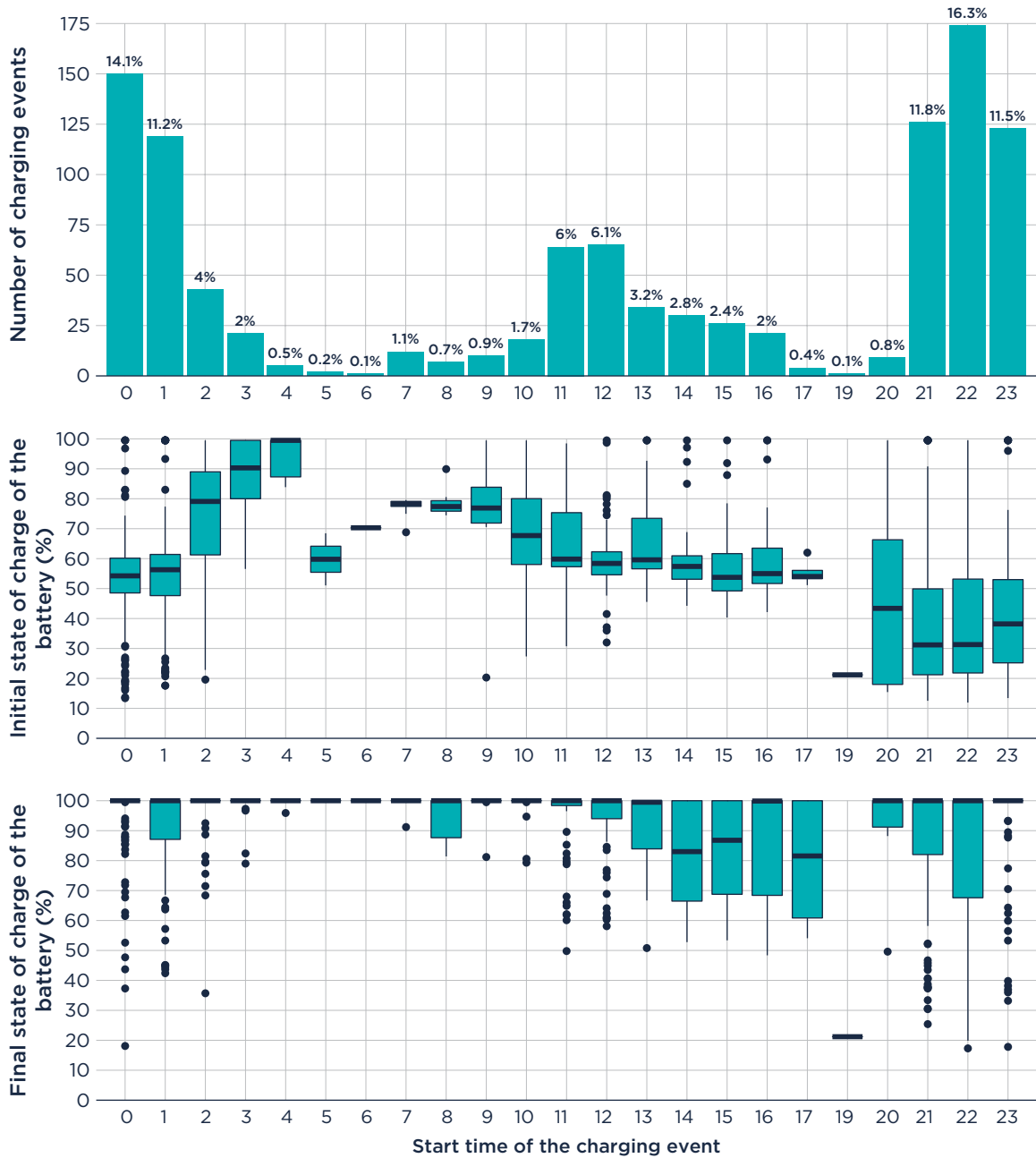
Figure 16. Battery charging strategy. The top panel displays the number of charging events per start time. The last two panels show the distribution of the percentage of energy available in the battery, also according to the start time of the charging event.
