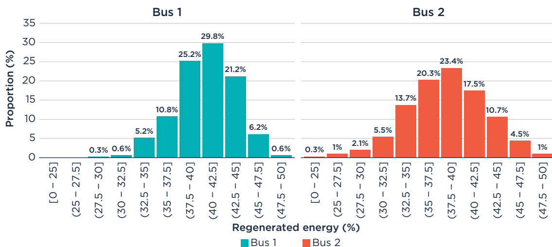
Figure 10. Distribution of the daily regenerated energy percentage
