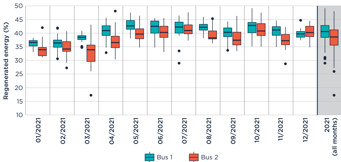
Figure 11. Distribution of daily energy regenerated by braking in each monitored month, aggregated for 2021
