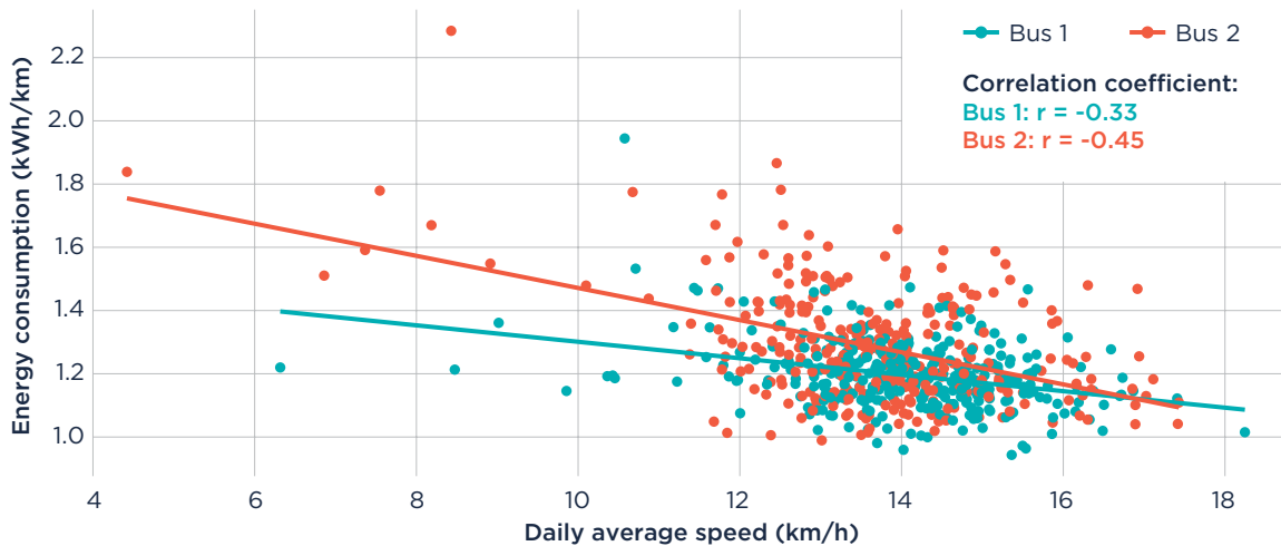
Figure 9. Relationship between daily energy consumption (kWh/km) and average operating speed (km/h) for each bus
