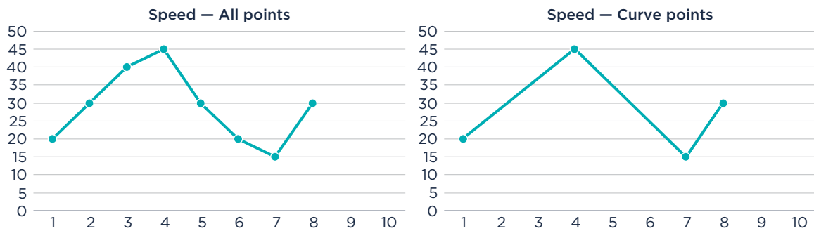
Figure 18. Collecting all speed data points versus collecting critical points (curve points). Adapted from Cawse (2022).
