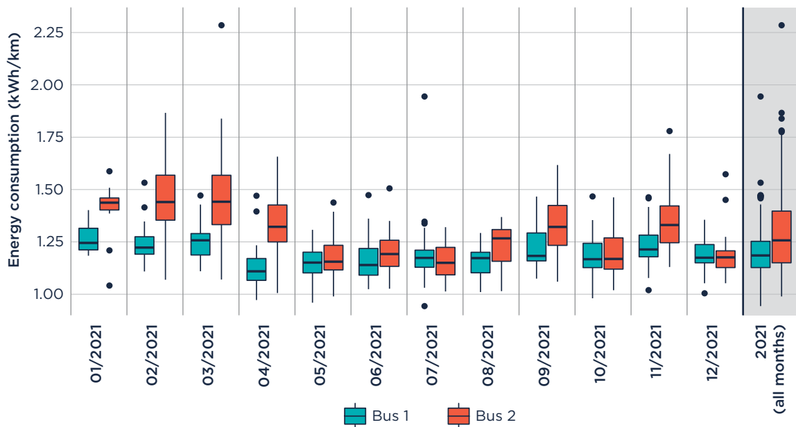
Figure 6. Daily energy consumption per kilometer over the monitored months, aggregated for 2021
