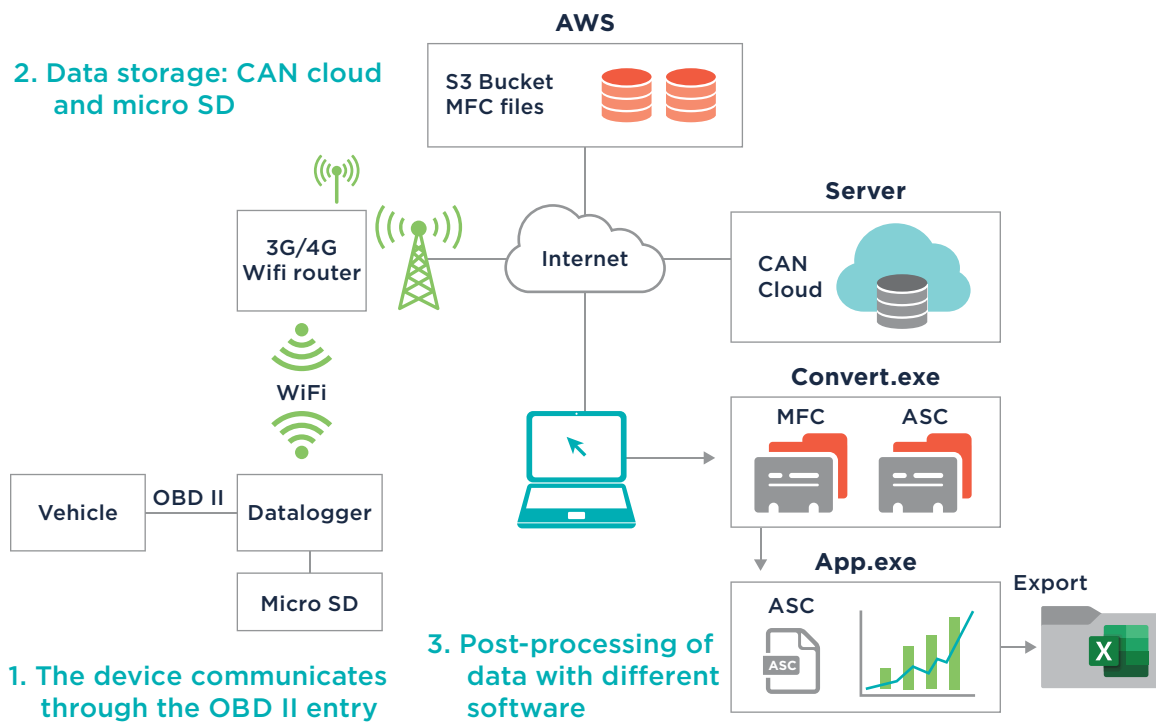
Figure 17. Data collection and storage structure for monitored electric vehicles
