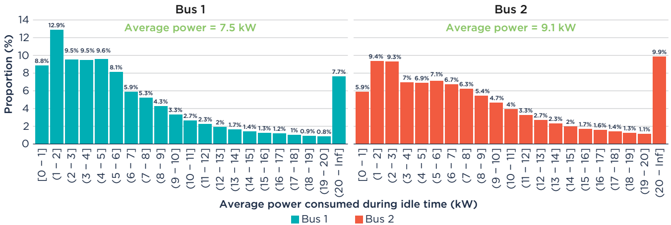
Figure 14. Distribution of power consumption (in kW) during idle time
