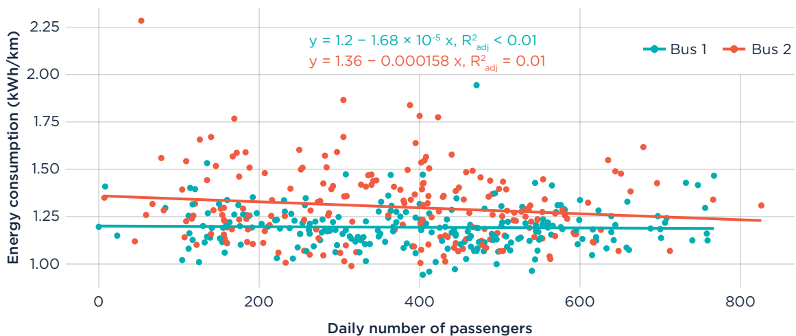
Figure 20. Relationship between energy consumption and the daily number of passengers
